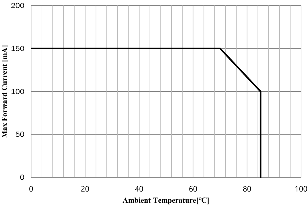
FIG 8. Max. Forward current vs Ambient Temperature (Rth J-S : 13.0°C/W)
