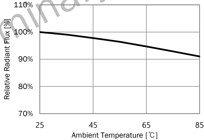
Fig 4. Relative Radiant Flux vs Ambient Temperature
