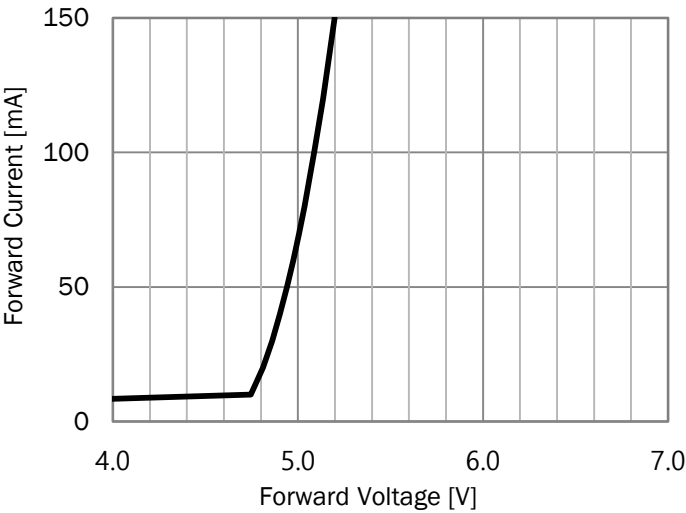
FIG 1. Forward Current vs. Forward Voltage
